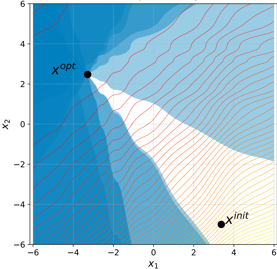
28 Discus with 6+n/2 constraints, instance=6
