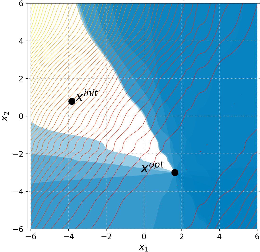
28 Discus with 6+n/2 constraints, instance=5
