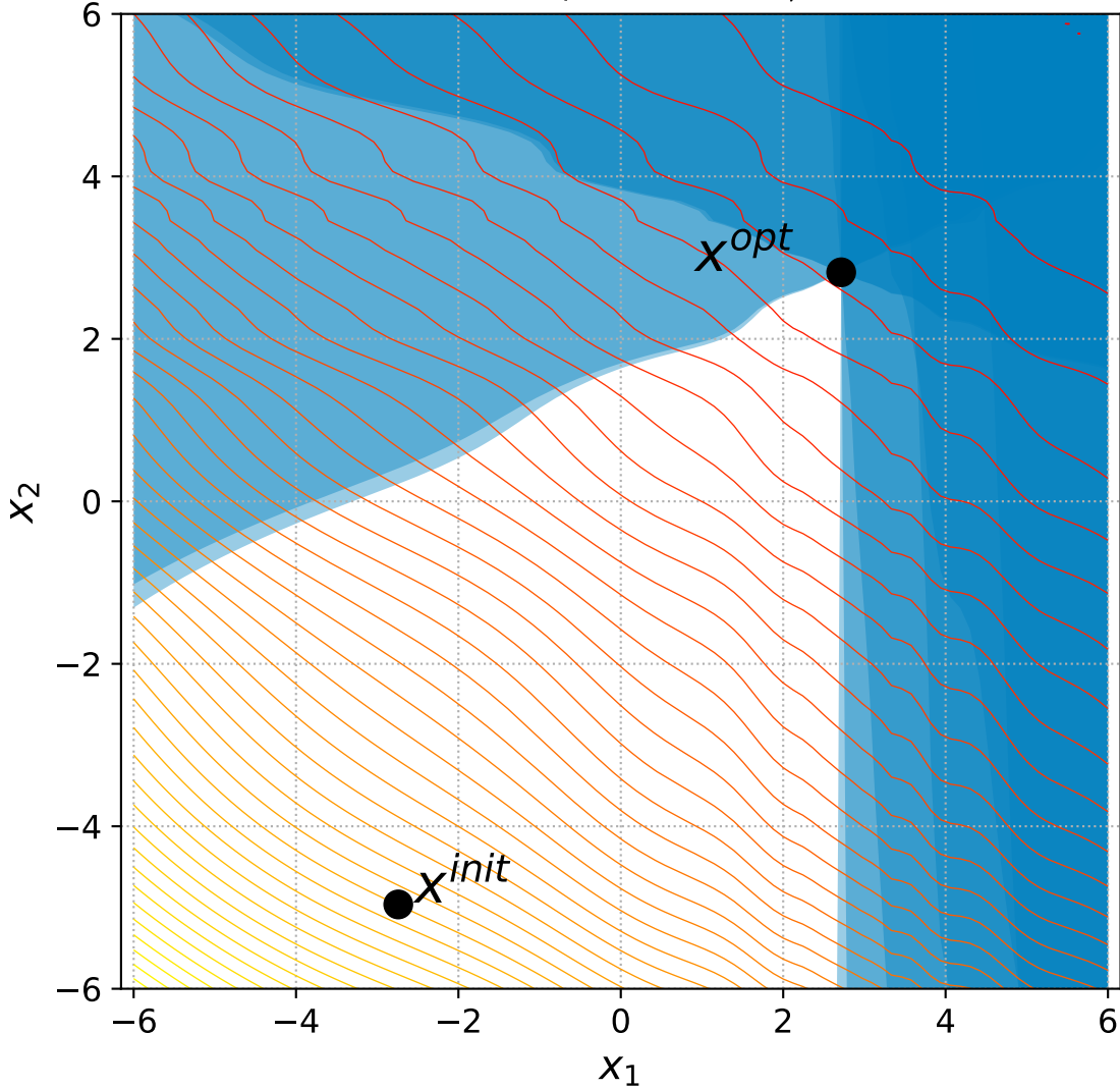
28 Discus with 6+n/2 constraints, instance=4
