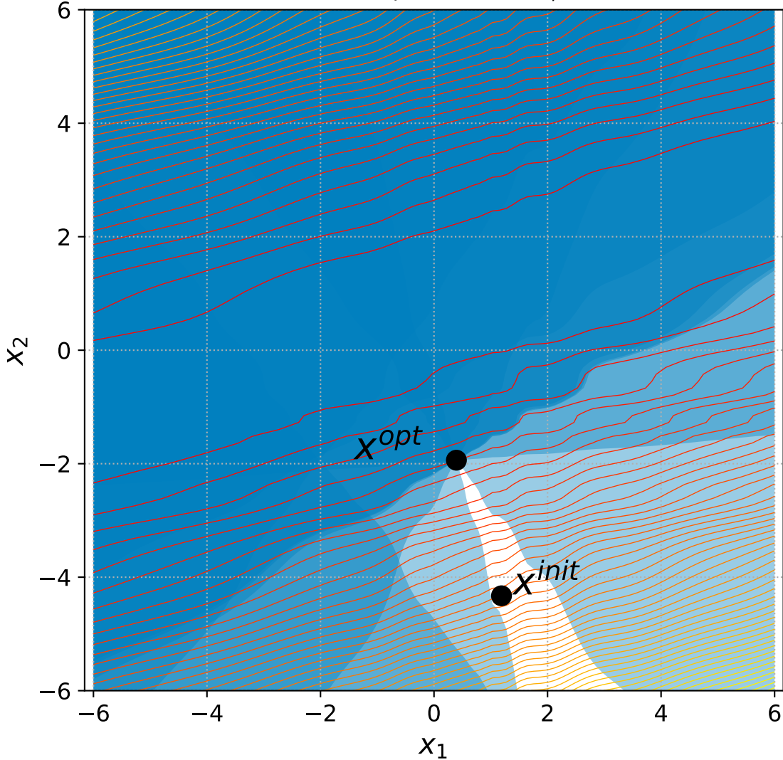
28 Discus with 6+n/2 constraints, instance=1
