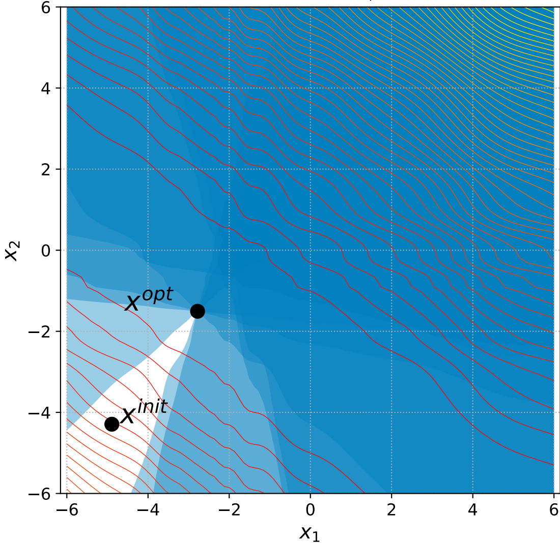
27 Discus with 6 constraints, instance=13
