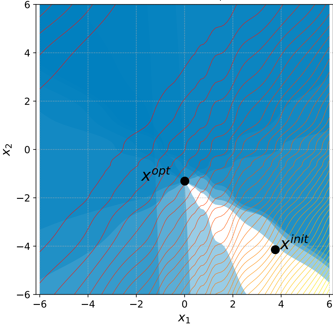
27 Discus with 6 constraints, instance=12
