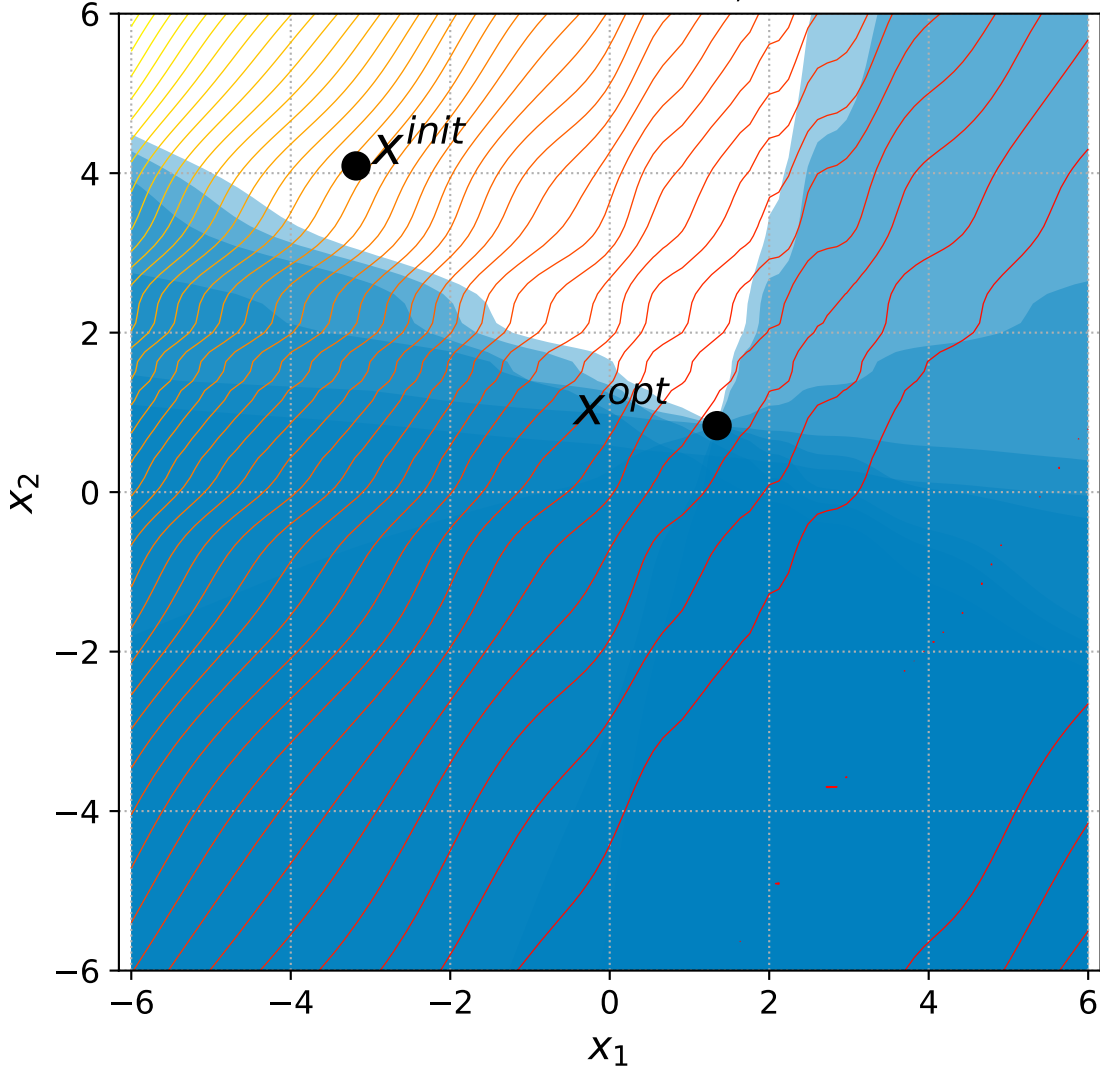
27 Discus with 6 constraints, instance=8
