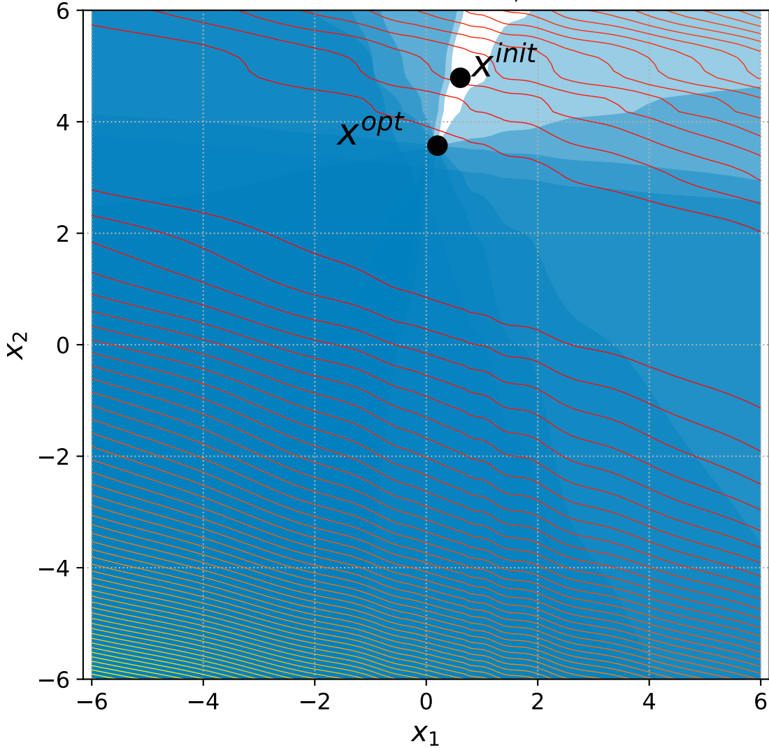
27 Discus with 6 constraints, instance=5
