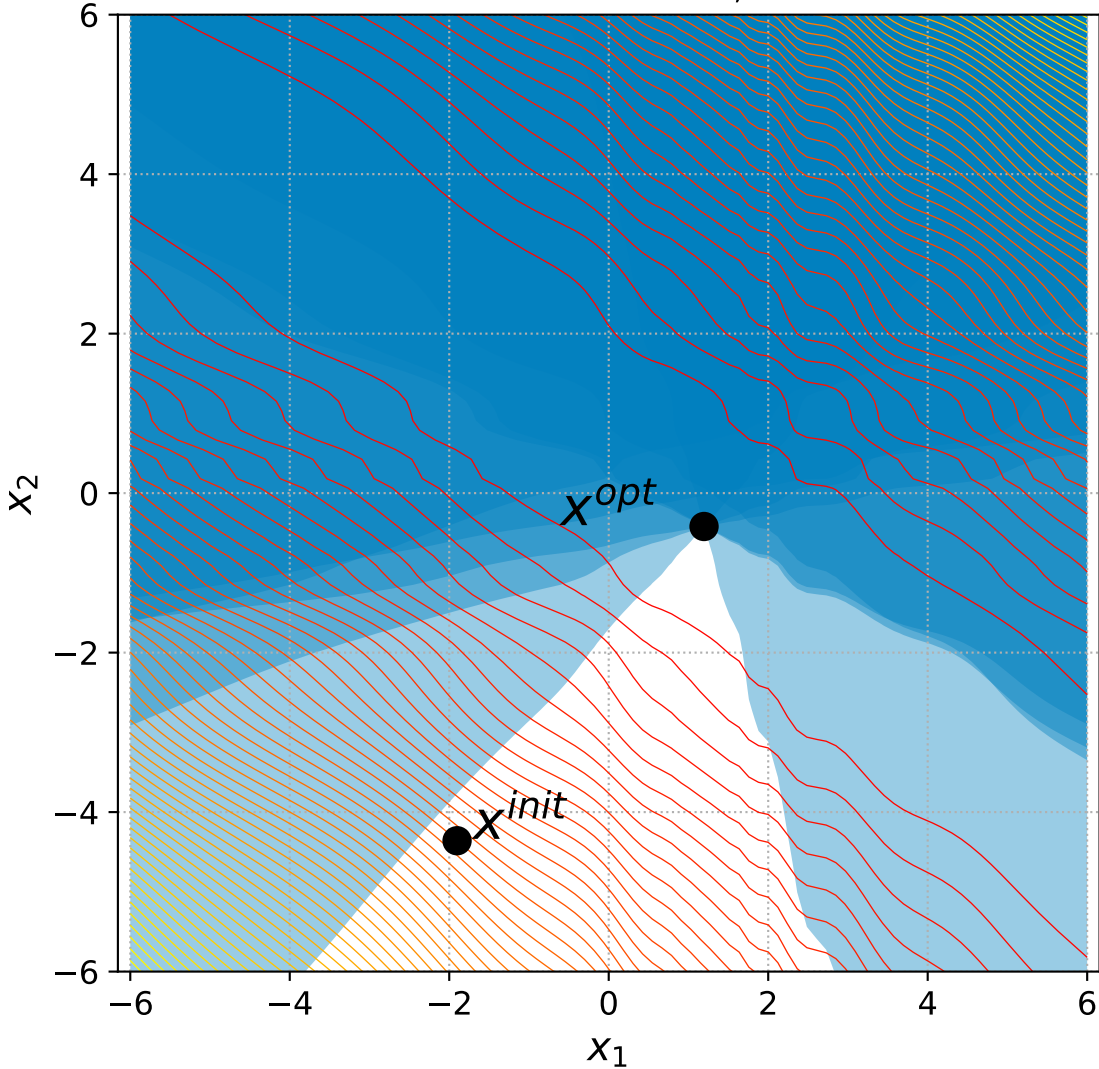
27 Discus with 6 constraints, instance=2
