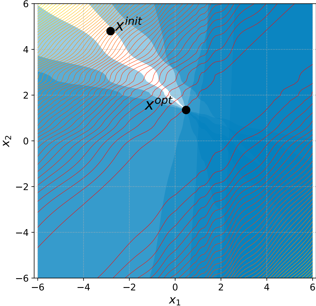
27 Discus with 6 constraints, instance=1
