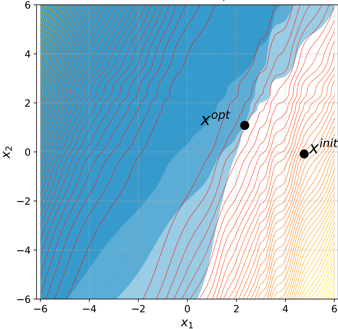
26 Discs with 2 constraints, instance=15
