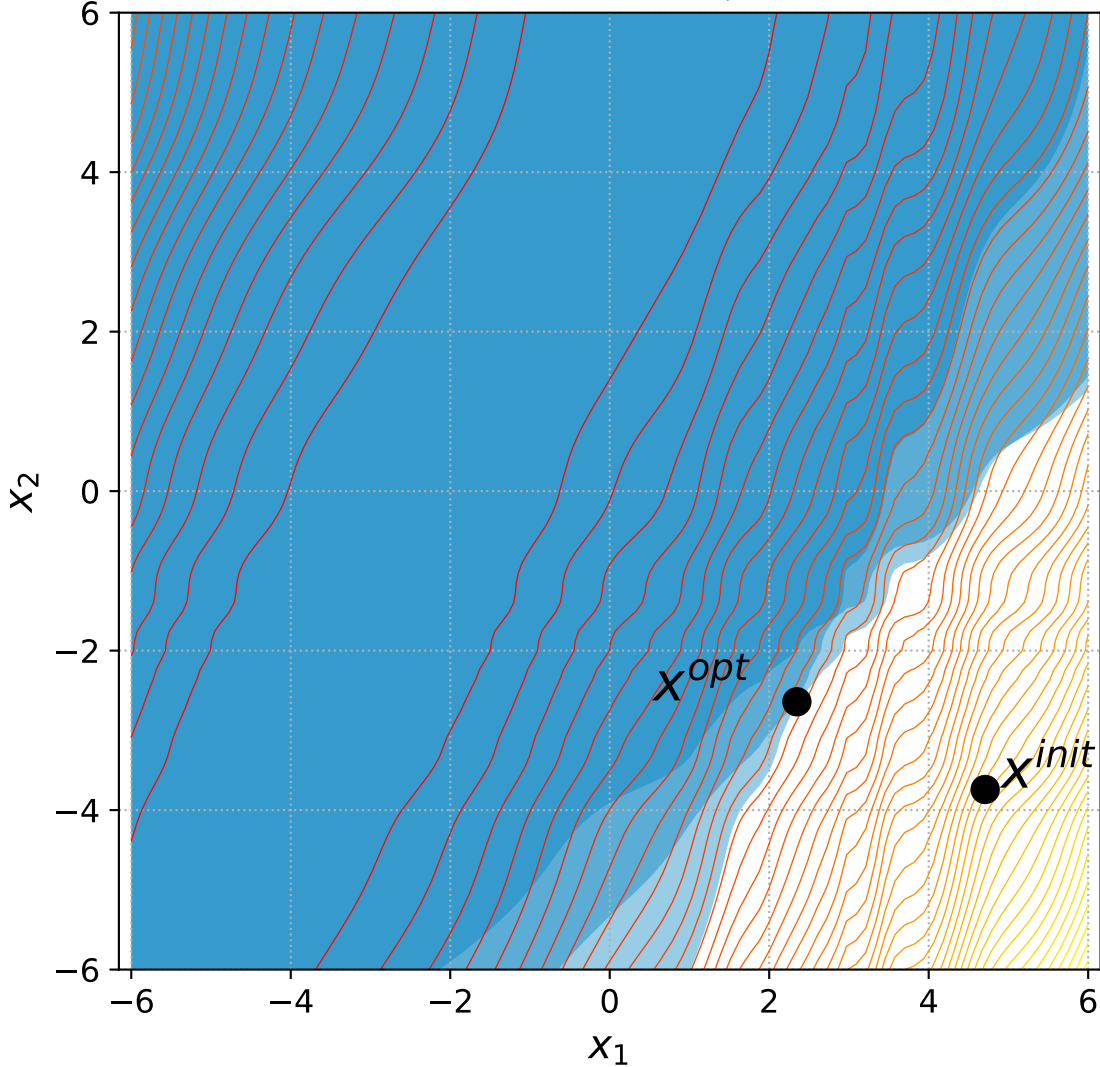
26 Discus with 2 constraints, instance=11
