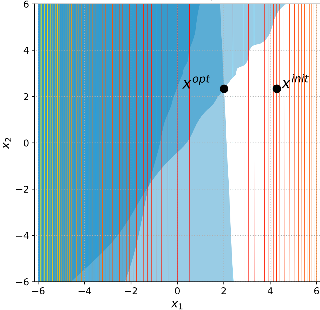
26 Discus with 2 constraints, instance=10
