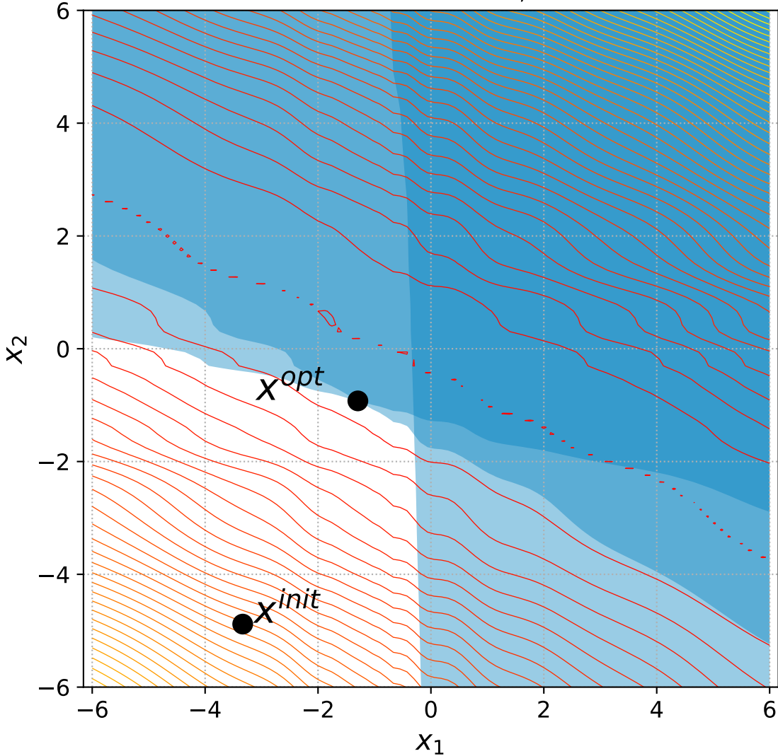
26 Discus with 2 constraints, instance=9
