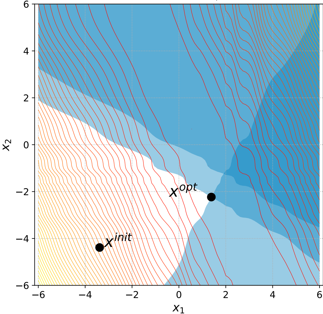
26 Discus with 2 constraints, instance=8
