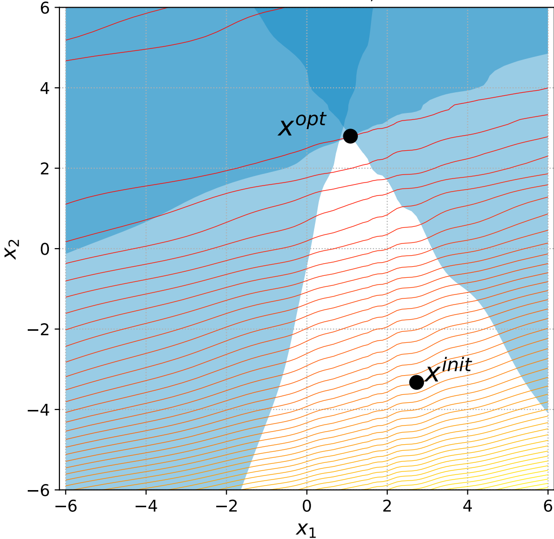
26 Discus with 2 constraints, instance=5
