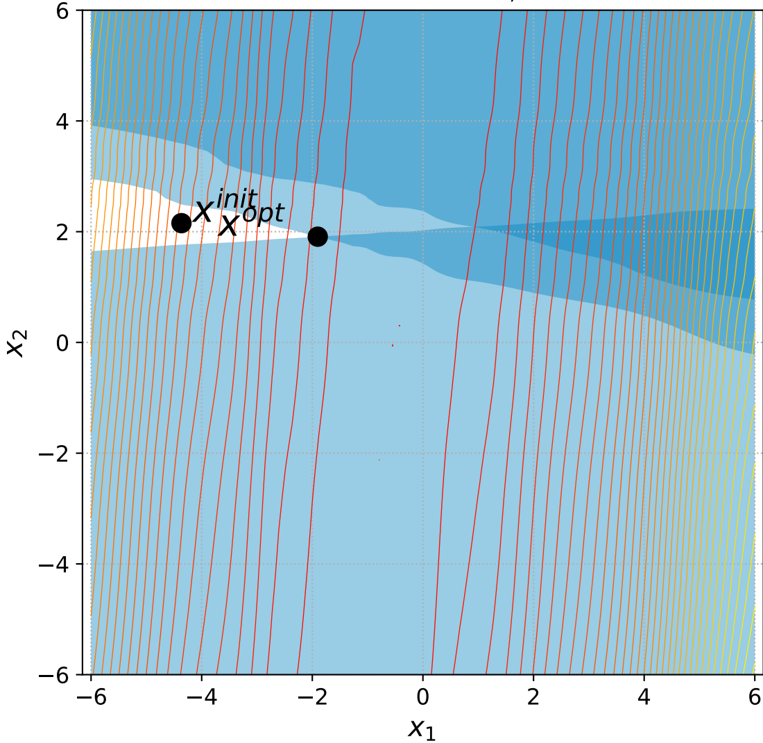
26 Discus with 2 constraints, instance=4
