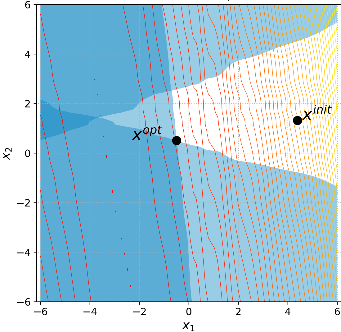
26 Discus with 2 constraints, instance=3
