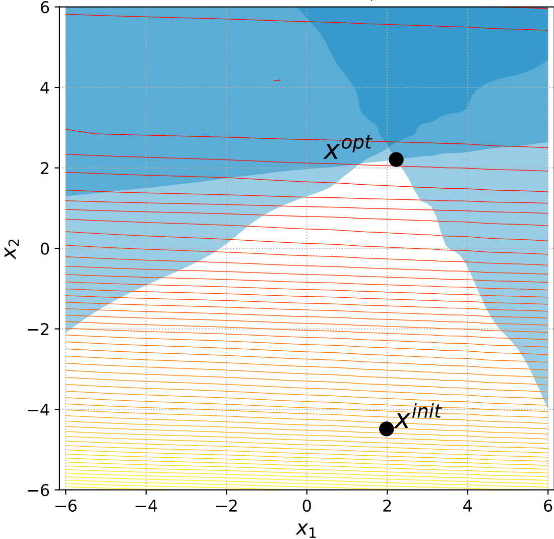
26 Discus with 2 constraints, instance=2
