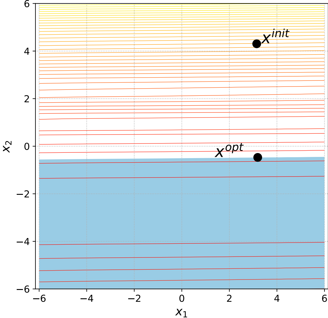
25 Discus with 1 constraint, instance=15
