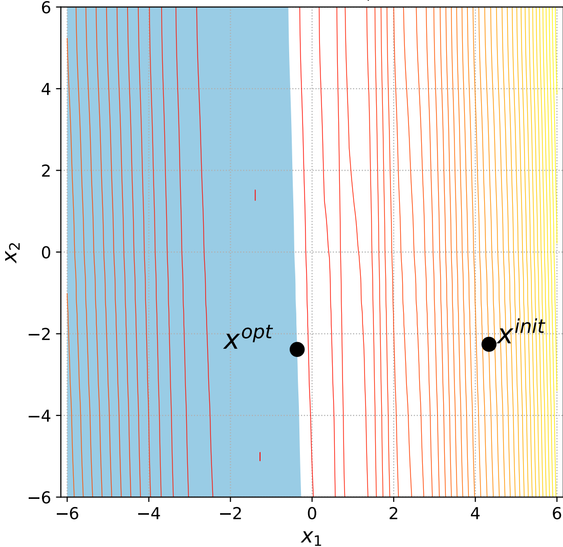
25 Discs with 1 constraint, instance=14
