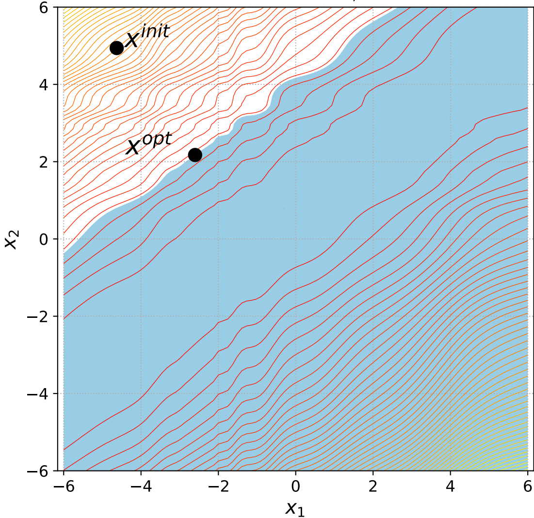
25 Discus with 1 constraint, instance=9
