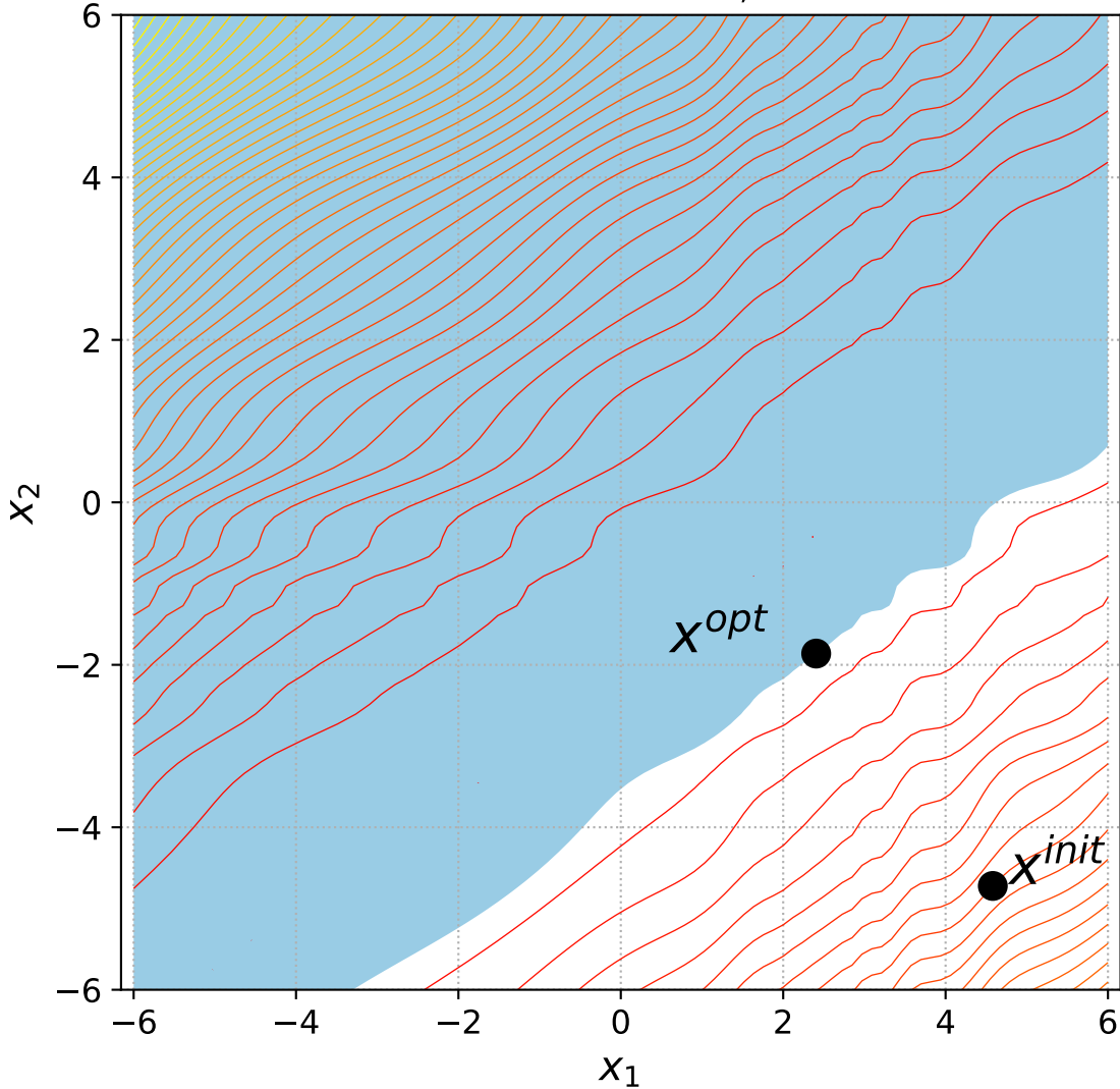
25 Discus with 1 constraint, instance=8
