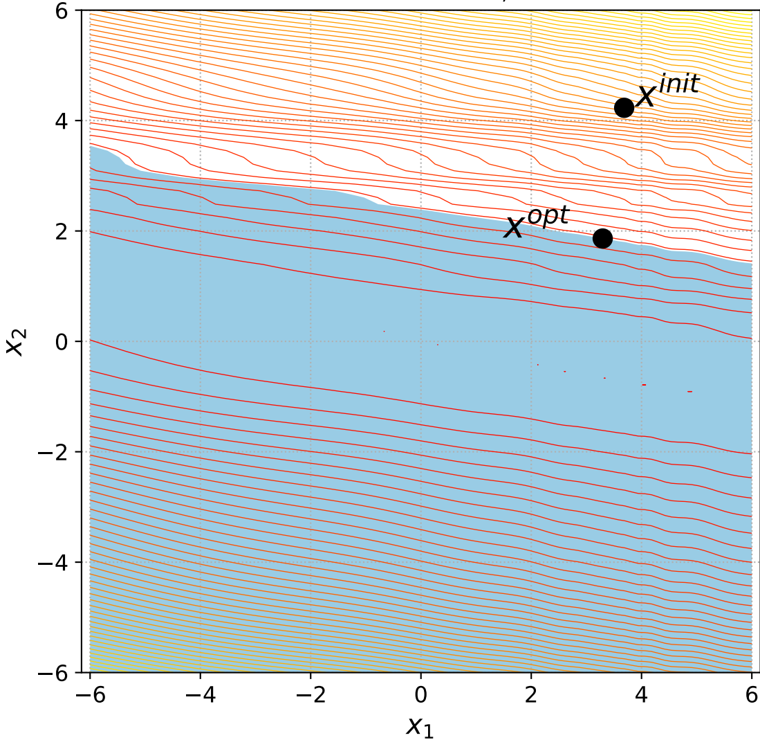
25 Discus with 1 constraint, instance=7
