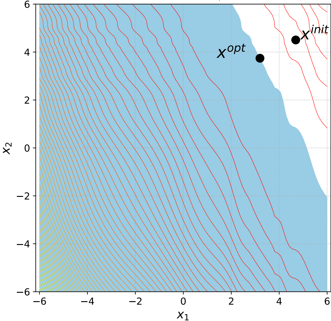
25 Discus with 1 constraint, instance=6
