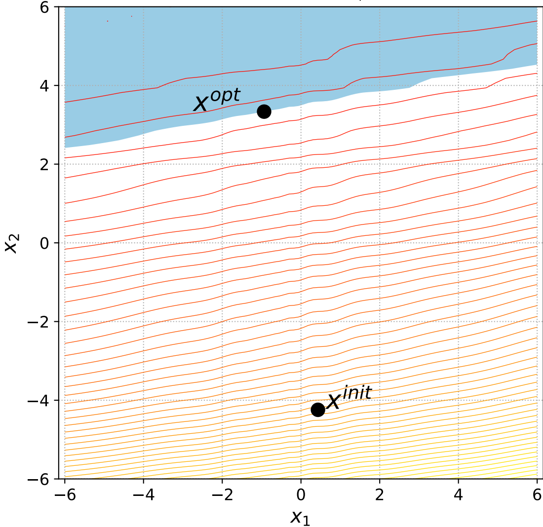
25 Discus with 1 constraint, instance=3
