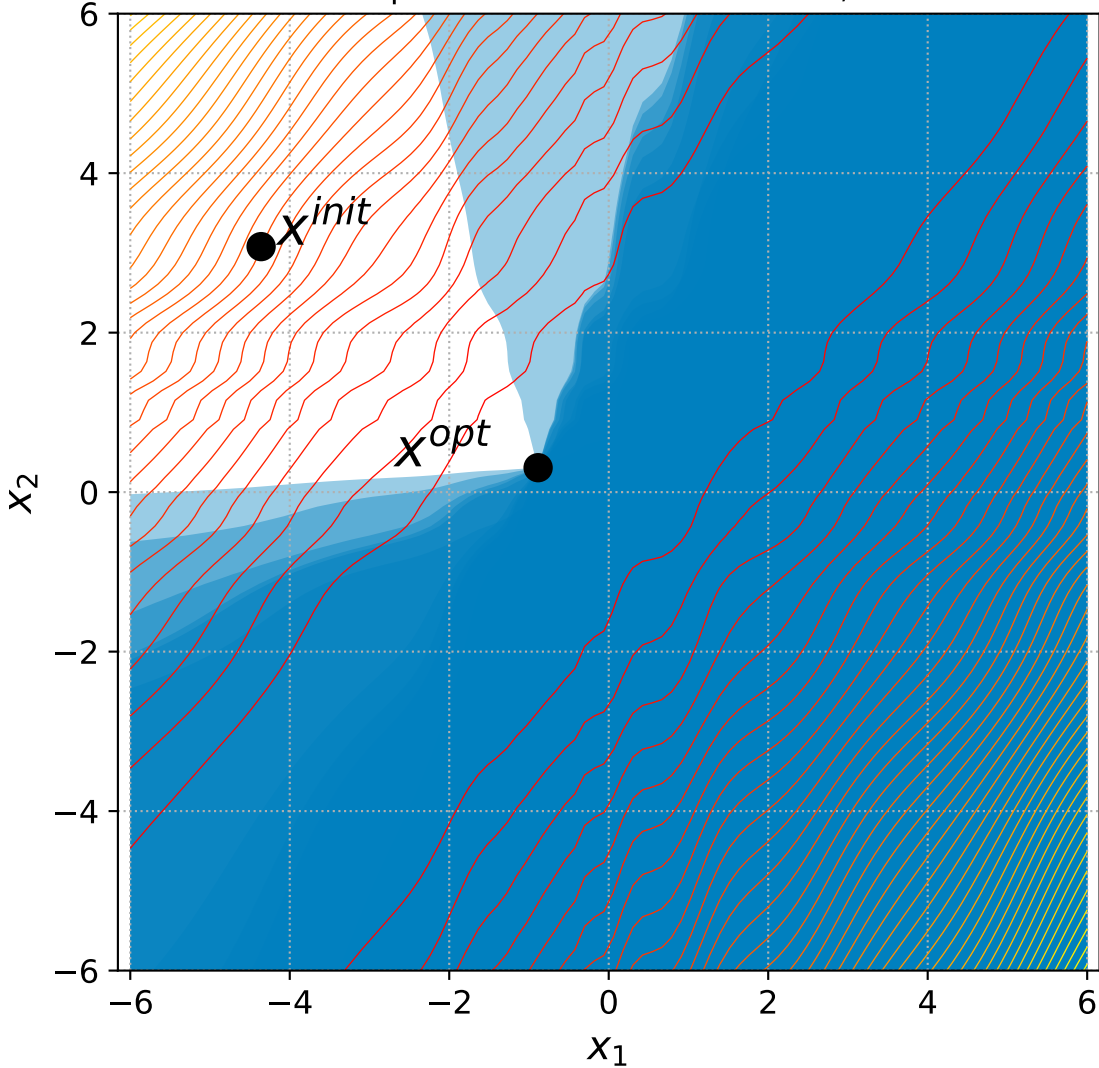
24 Rotated Ellipsoid with 6+3n constraints, instance=15
