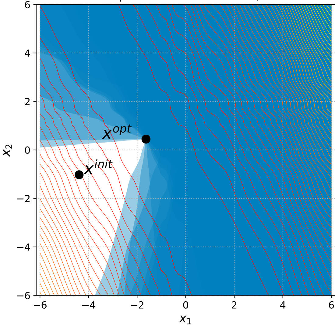
24 Rotated Ellipsoid with 6+3n constraints, instance=13
