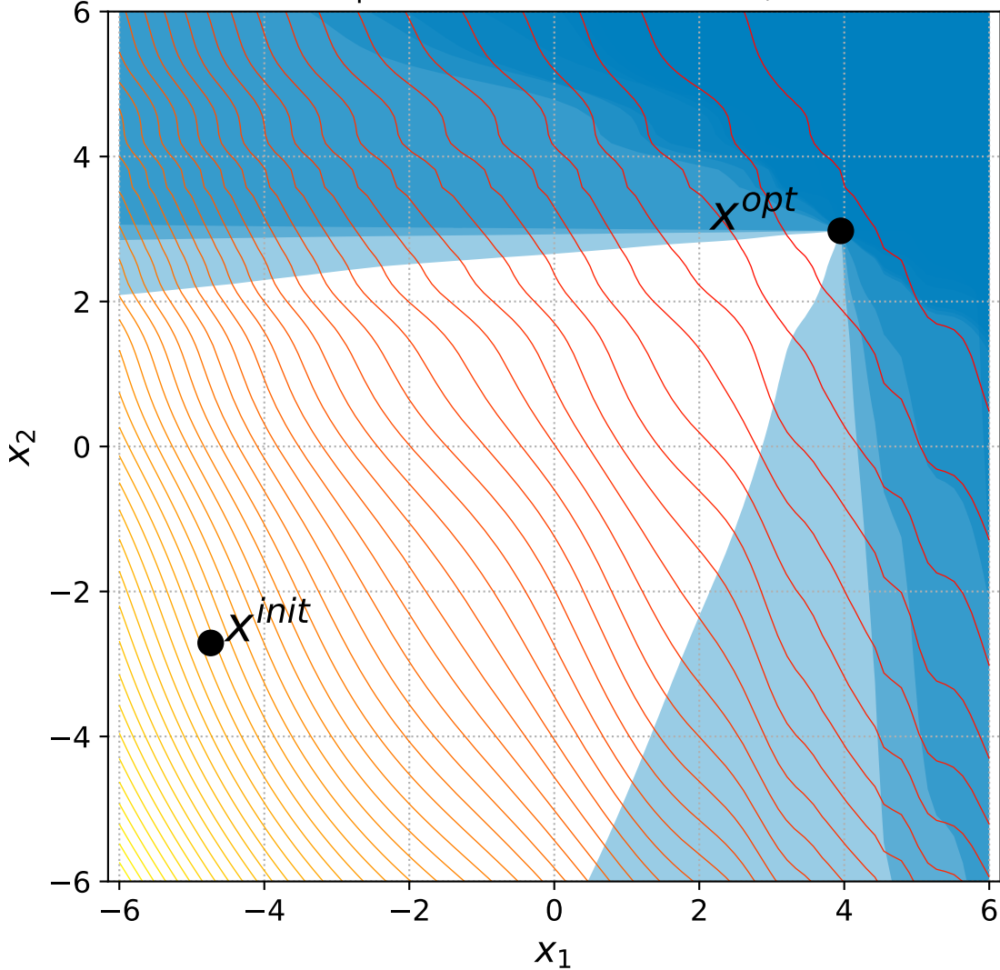
24 Rotated Ellipsoid with 6+3n constraints, instance=12
