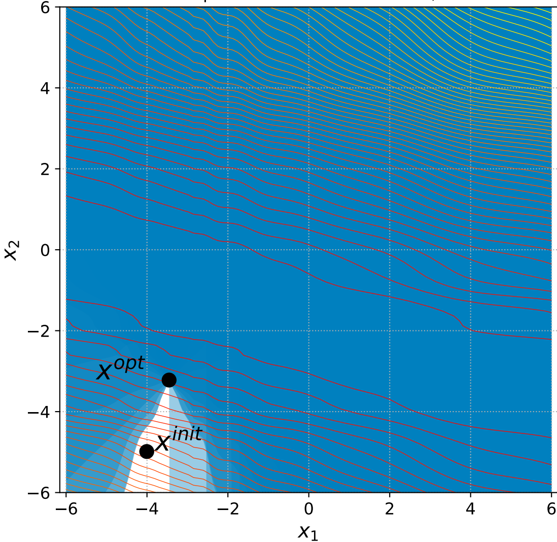
24 Rotated Ellipsoid with 6+3n constraints, instance=9
