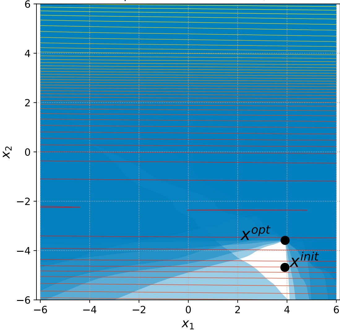
24 Rotated Ellipsoid with 6+3n constraints, instance=7
