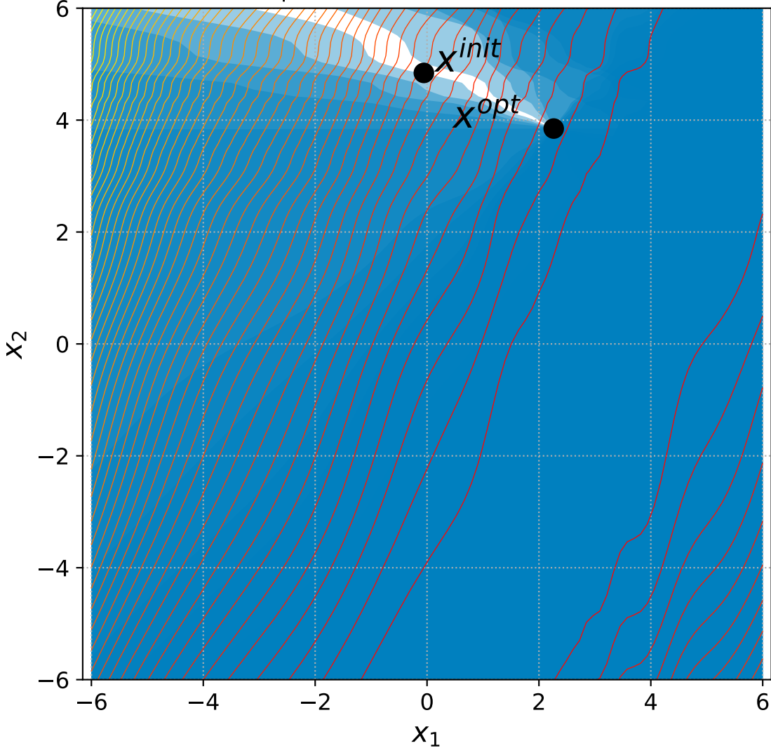
24 Rotated Ellipsoid with 6+3n constraints, instance=6
