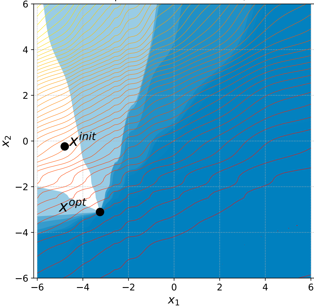
24 Rotated Ellipsoid with 6+3n constraints, instance=5
