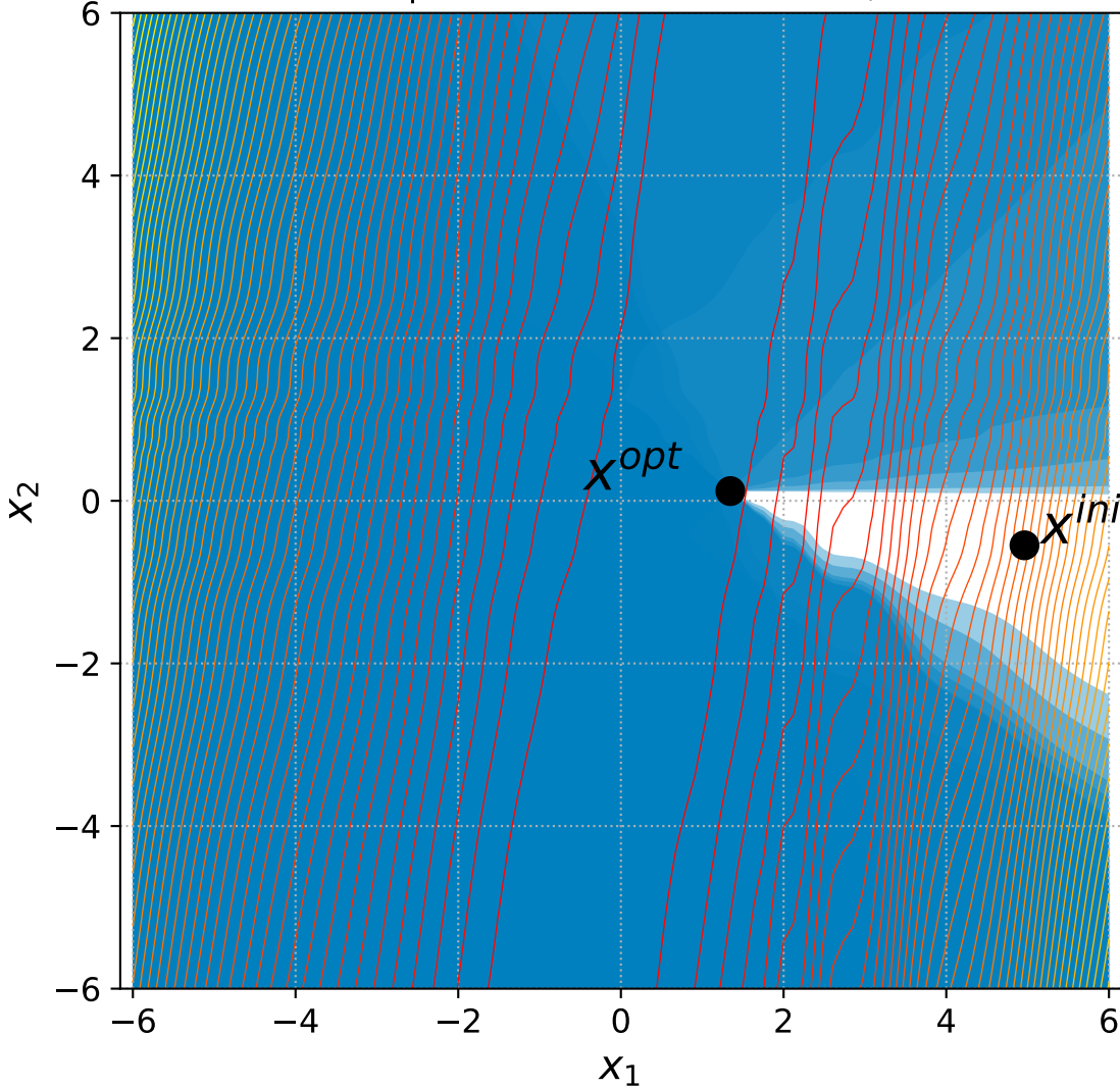
24 Rotated Ellipsoid with 6+3n constraints, instance=2
