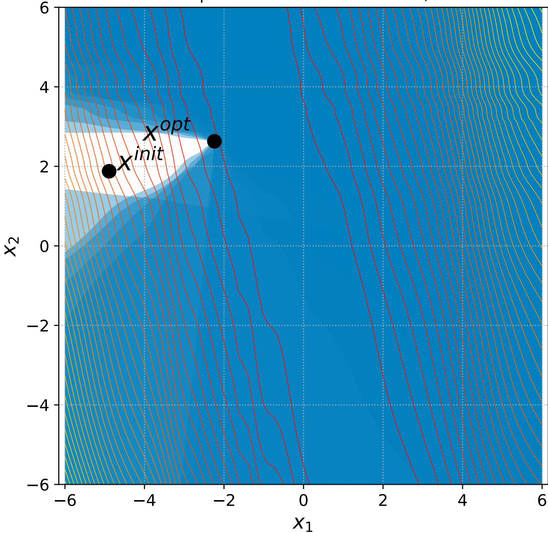
24 Rotated Ellipsoid with 6+3n constraints, instance=1
