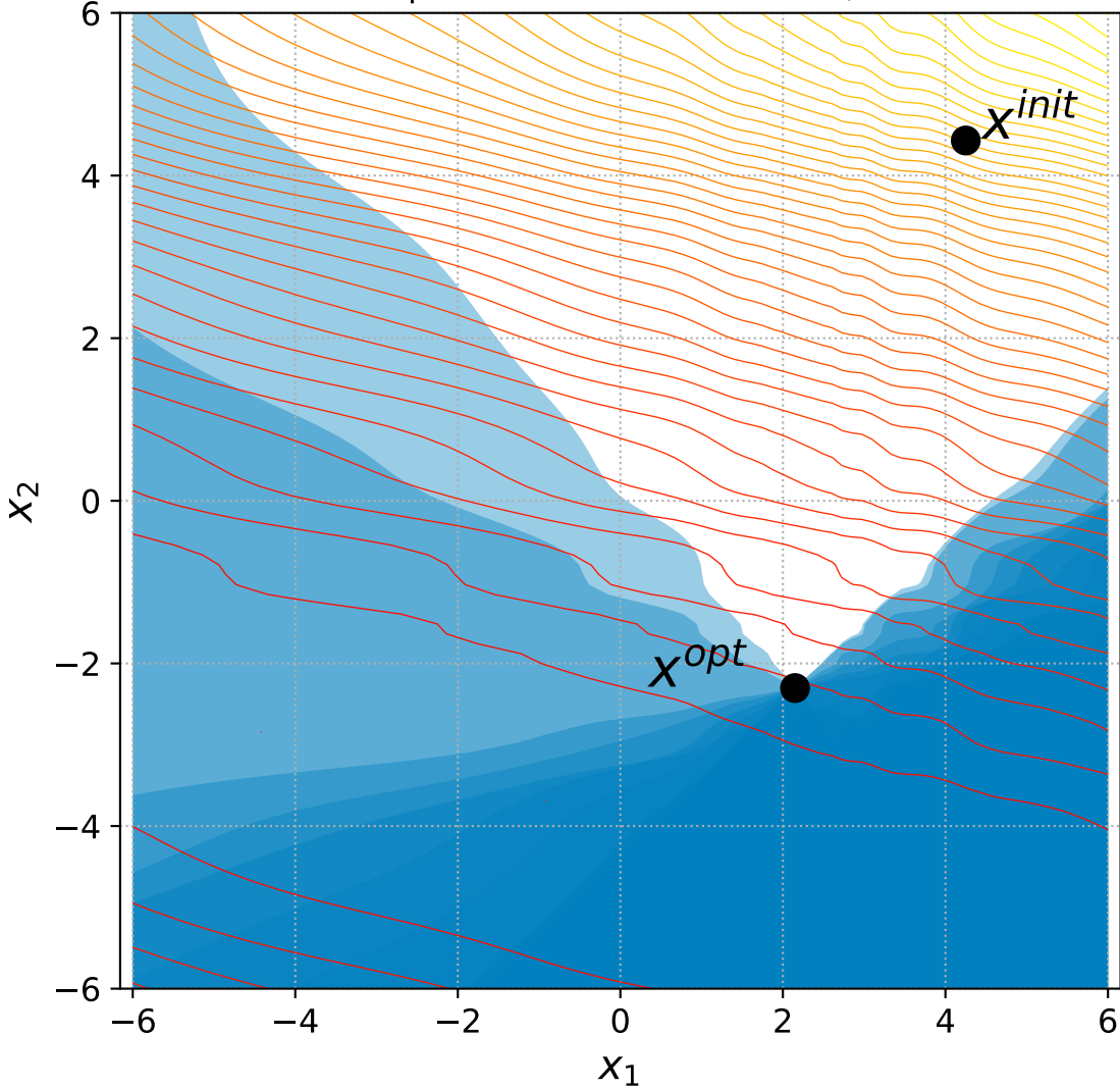
23 Rotated Ellipsoid with 6+n constraints, instance=15
