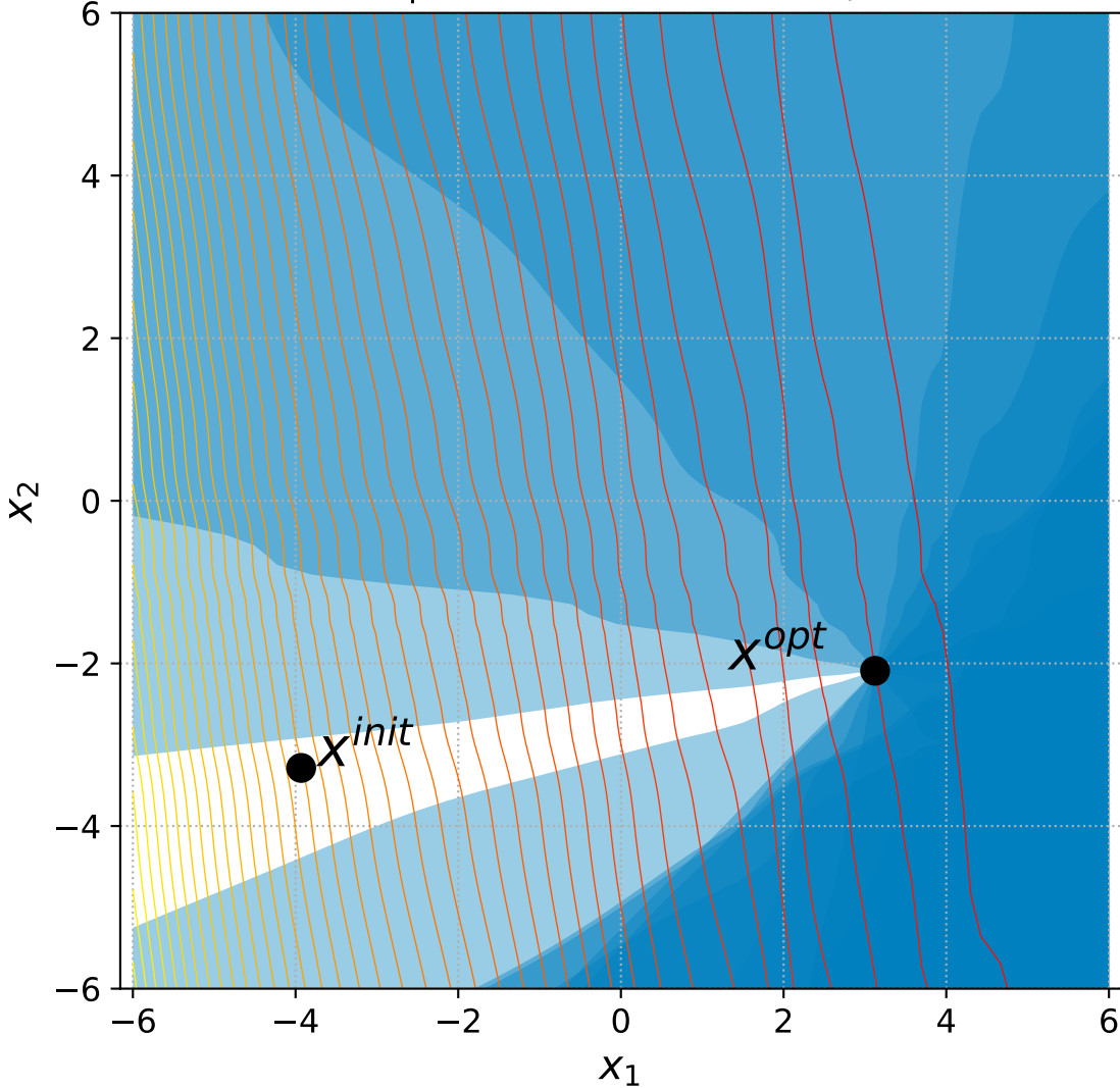
23 Rotated Ellipsoid with 6+n constraints, instance=14
