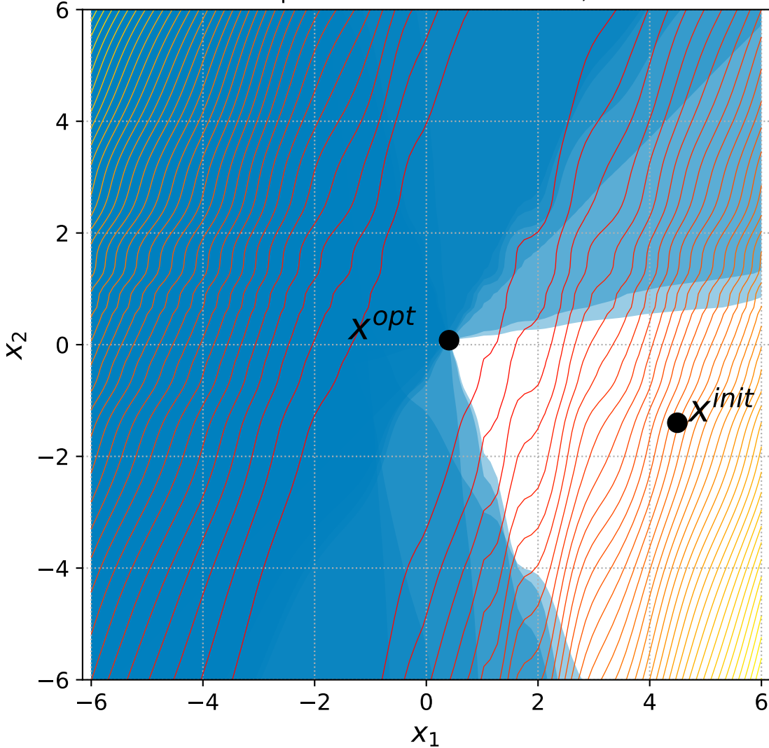
23 Rotated Ellipsoid with 6+n constraints, instance=13
