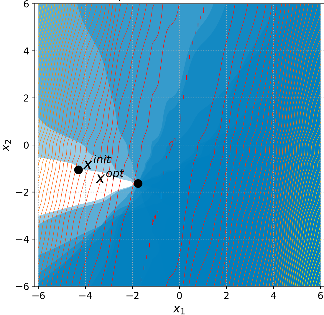
23 Rotated Ellipsoid with 6+n constraints, instance=12
