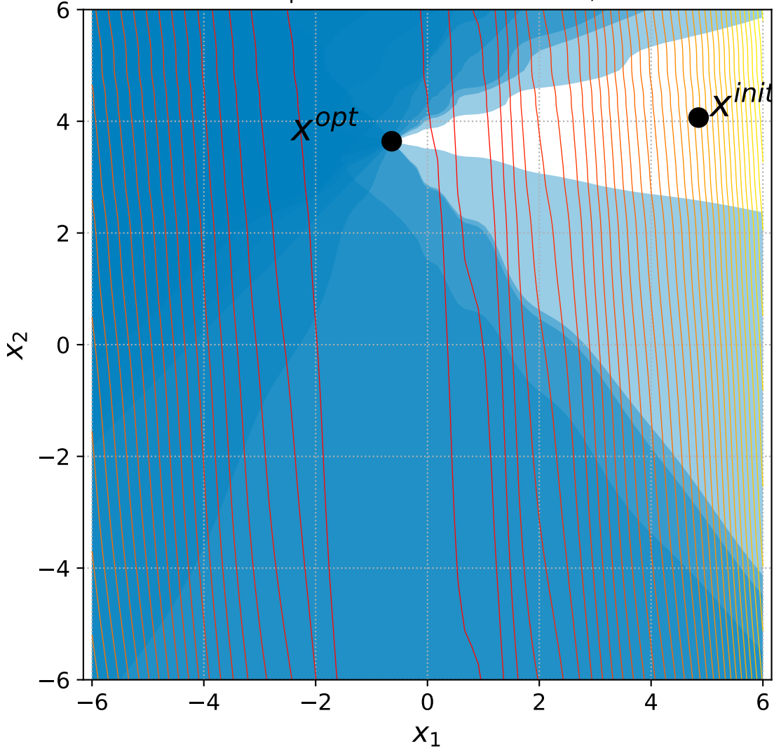
23 Rotated Ellipsoid with 6+n constraints, instance=9
