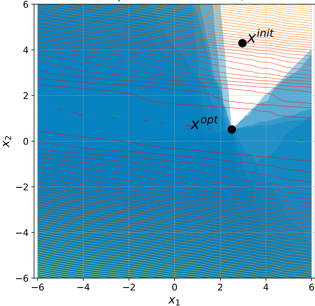
23 Rotated Ellipsoid with 6+n constraints, instance=8
