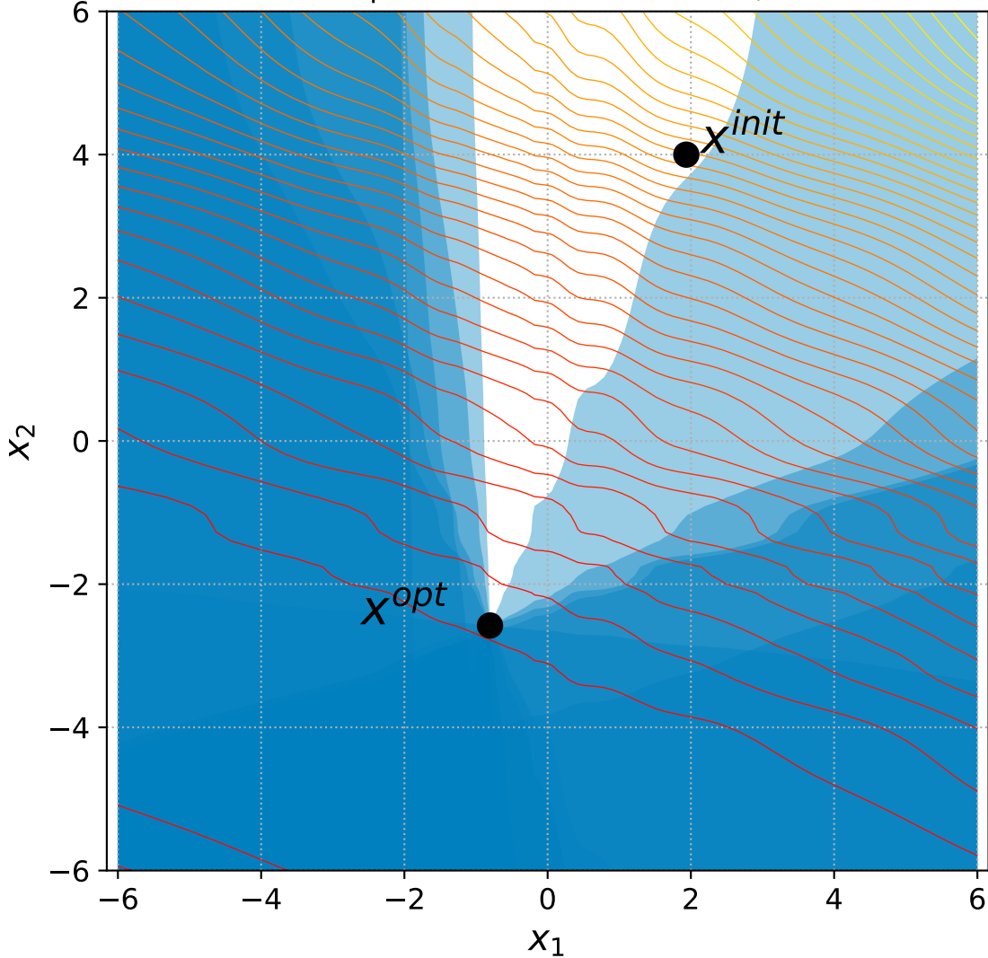
23 Rotated Ellipsoid with 6+n constraints, instance=6
