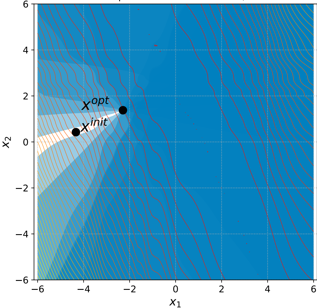
23 Rotated Ellipsoid with 6+n constraints, instance=4
