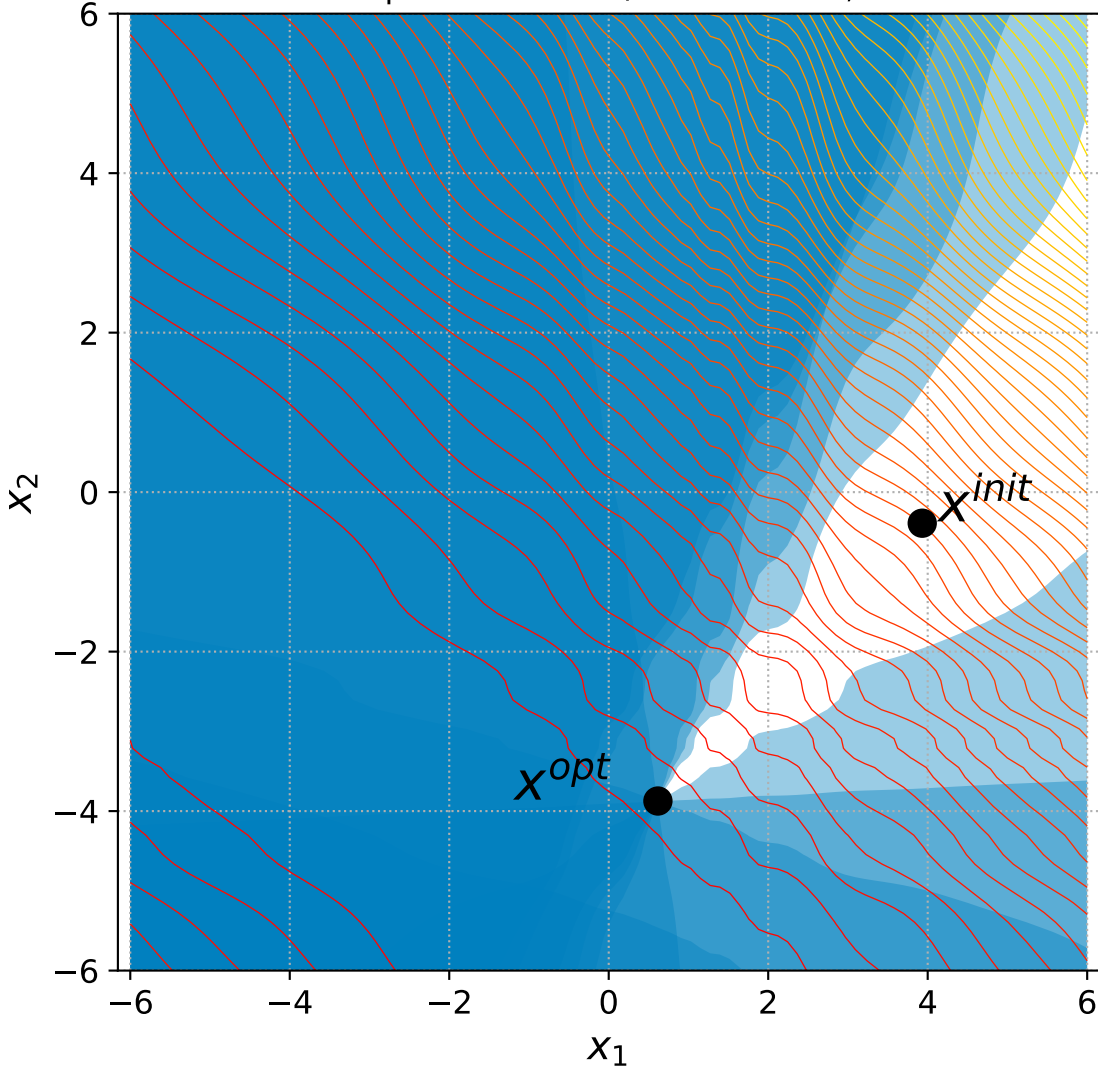
22 Rotated Ellipsoid with 6+n/2 constraints, instance=15
