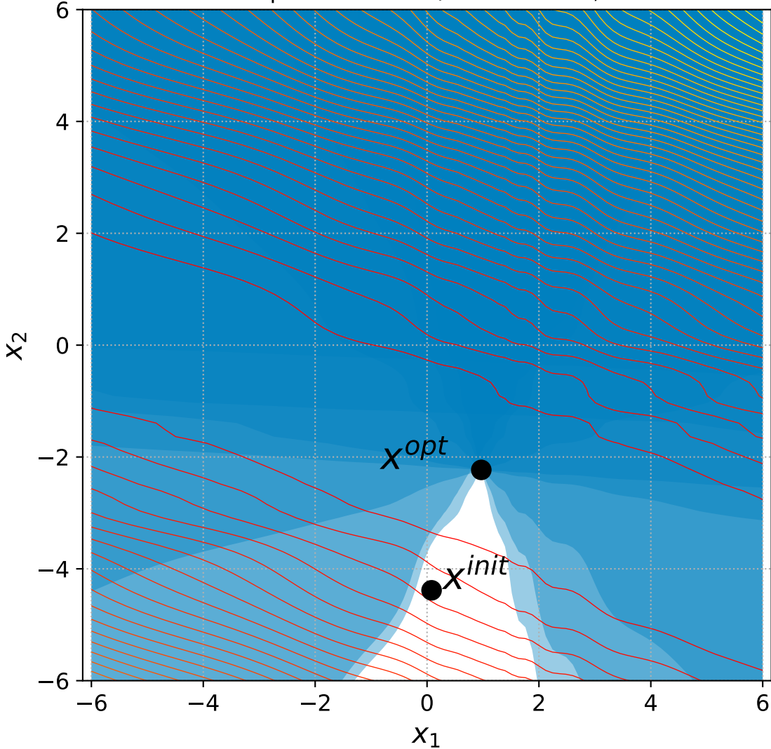
22 Rotated Ellipsoid with 6+n/2 constraints, instance=14
