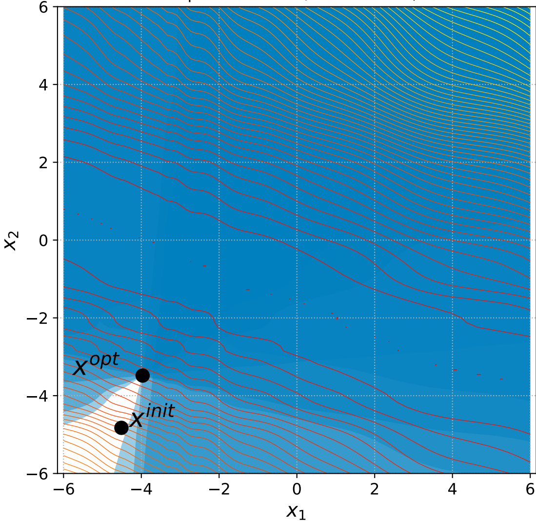
22 Rotated Ellipsoid with 6+n/2 constraints, instance=13
