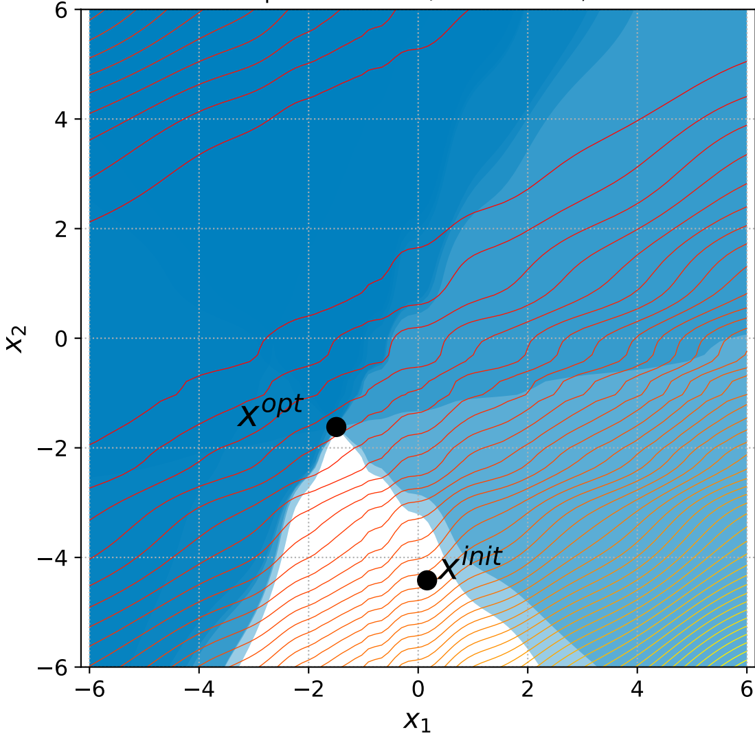
22 Rotated Ellipsoid with 6+n/2 constraints, instance=12
