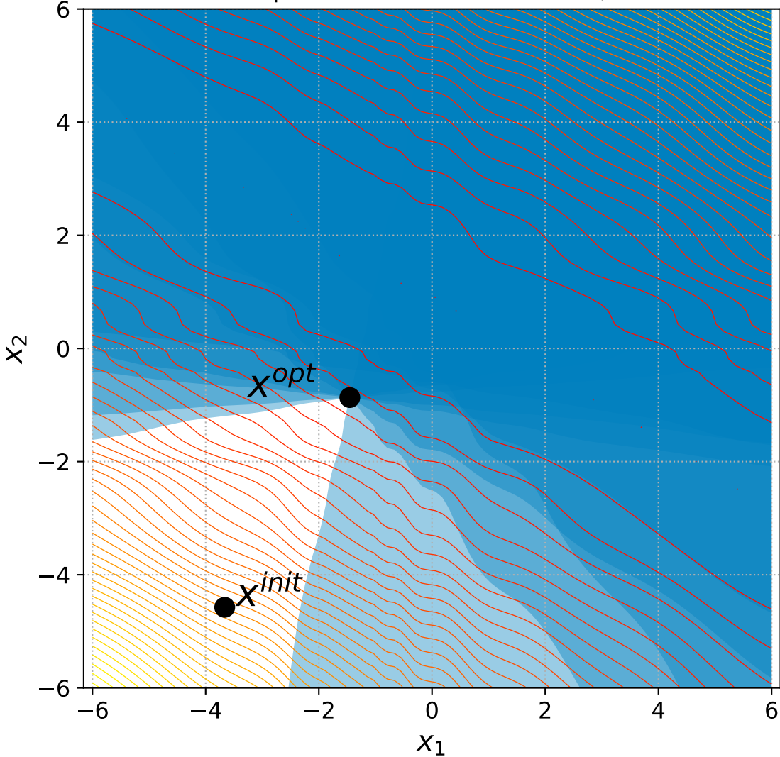
22 Rotated Ellipsoid with 6+n/2 constraints, instance=11
