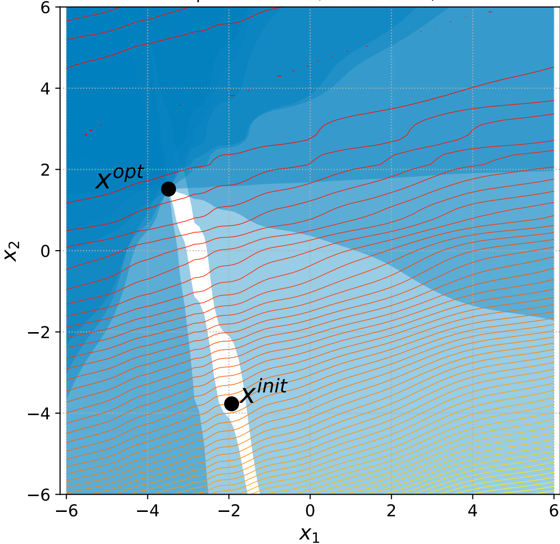
22 Rotated Ellipsoid with 6+n/2 constraints, instance=10
