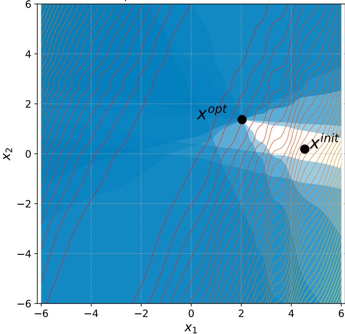
22 Rotated Ellipsoid with 6+n/2 constraints, instance=9
